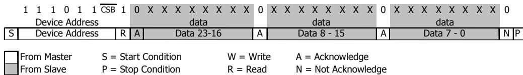
Figure 15: I 2 C answer from MS5607-B
