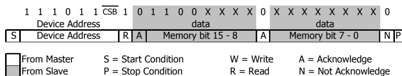
Figure 12: I 2 C answer from MS5607-B
